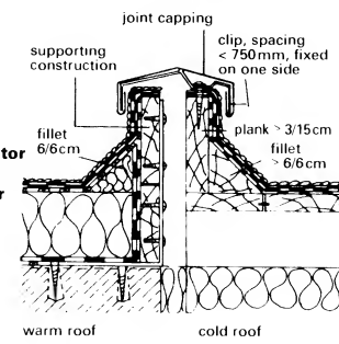
19 Movement joint with supporting construction and capping
